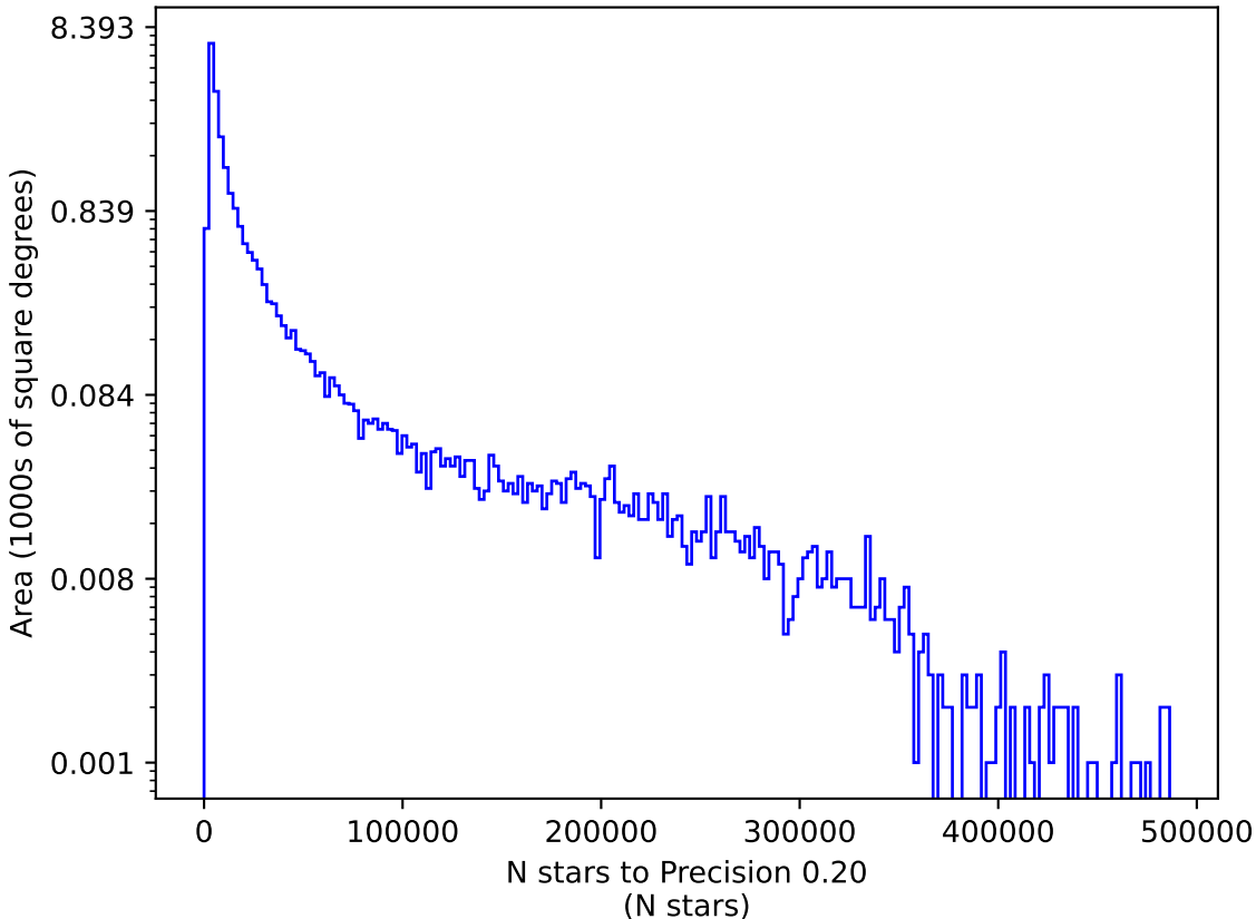
too_ignore_100_1v3.4_10yrs u: N stars to Precision 0.20
