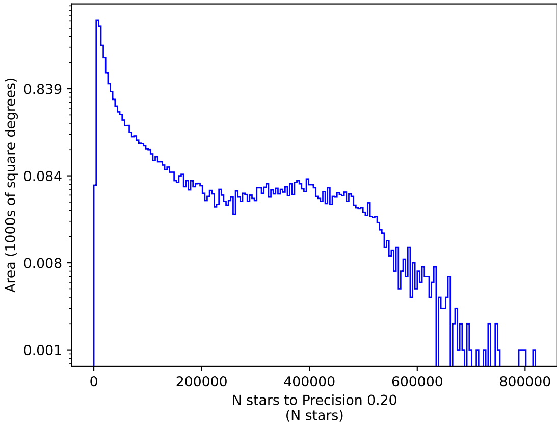
too_ignore_100_1v3.4_10yrs r: N stars to Precision 0.20
