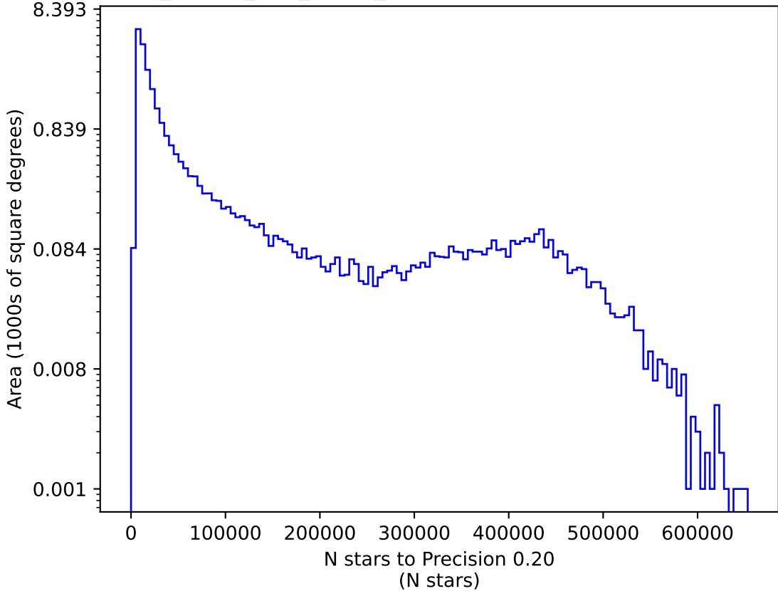
too_ignore_100_1v3.4_10yrs i: N stars to Precision 0.20
