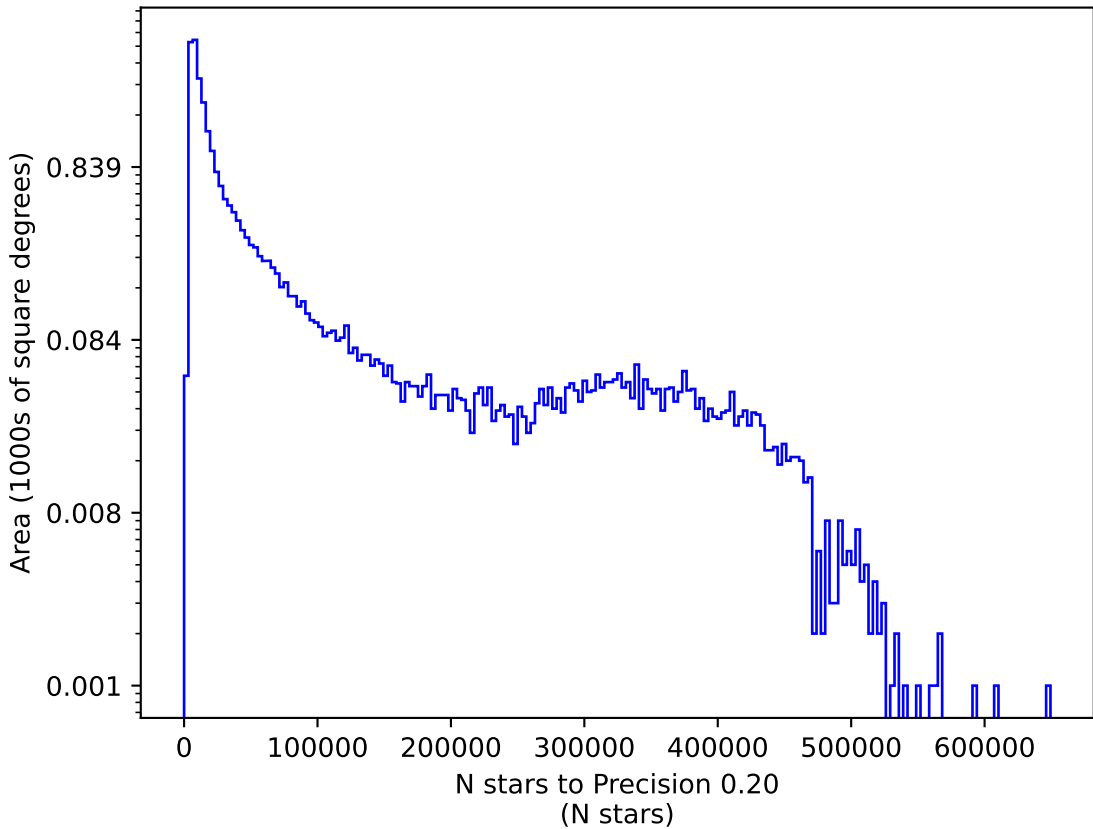
too_ignore_100_1v3.4_10yrs g: N stars to Precision 0.20
