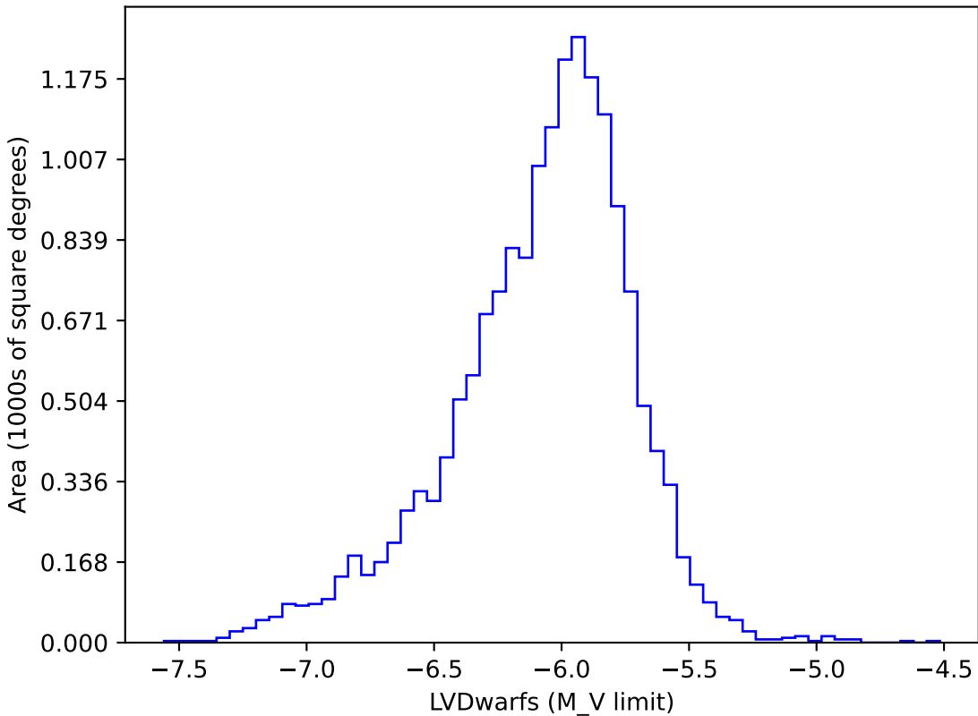
too_ignore_100_1v3.4_10yrs gi: LVDwarfs
