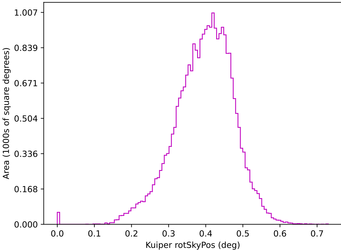
too_ignore_100_1v3.4_10yrs z: Kuiper rotSkyPos
