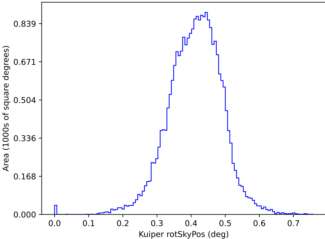
too_ignore_100_1v3.4_10yrs y: Kuiper rotSkyPos
