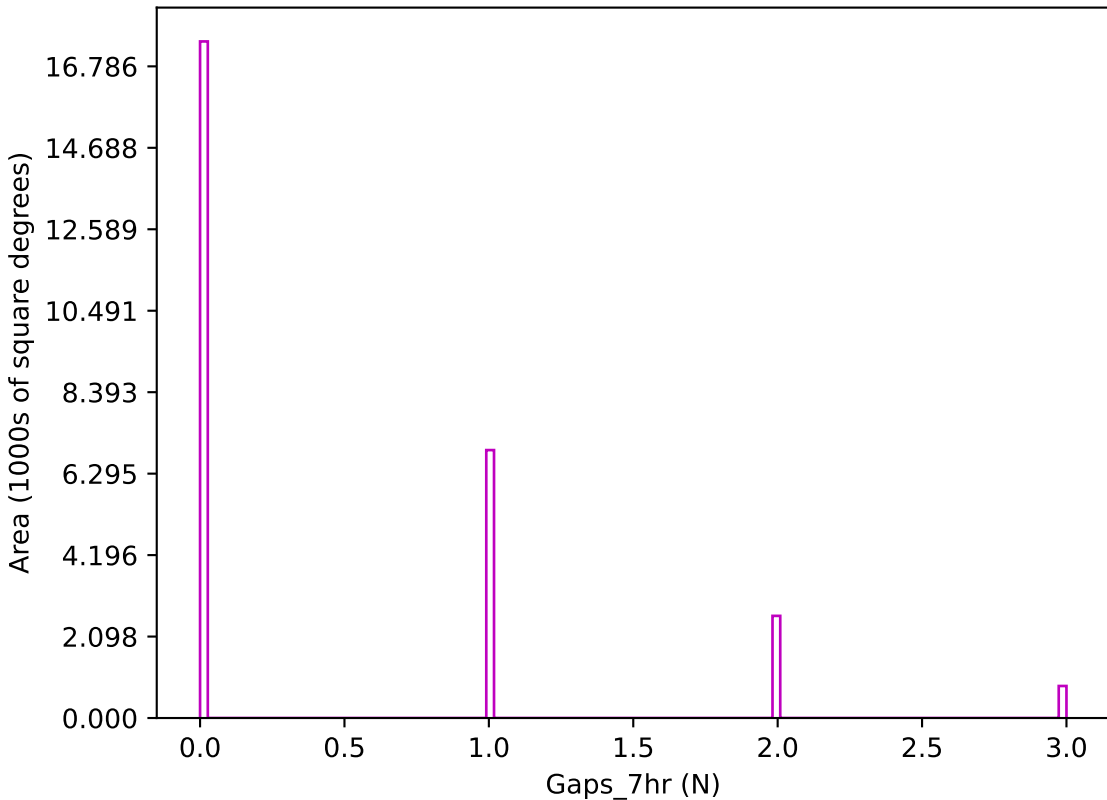
too_ignore_100_1v3.4_10yrs z band: Gaps_7hr
