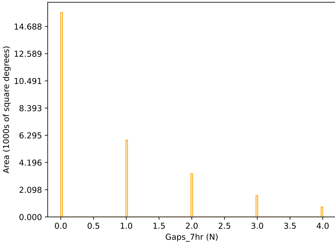
too_ignore_100_1v3.4_10yrs r band: Gaps_7hr
