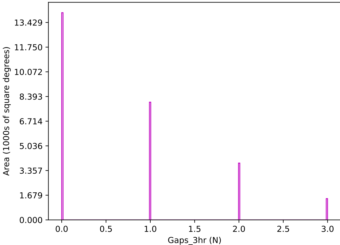
too_ignore_100_1v3.4_10yrs z band: Gaps_3hr
