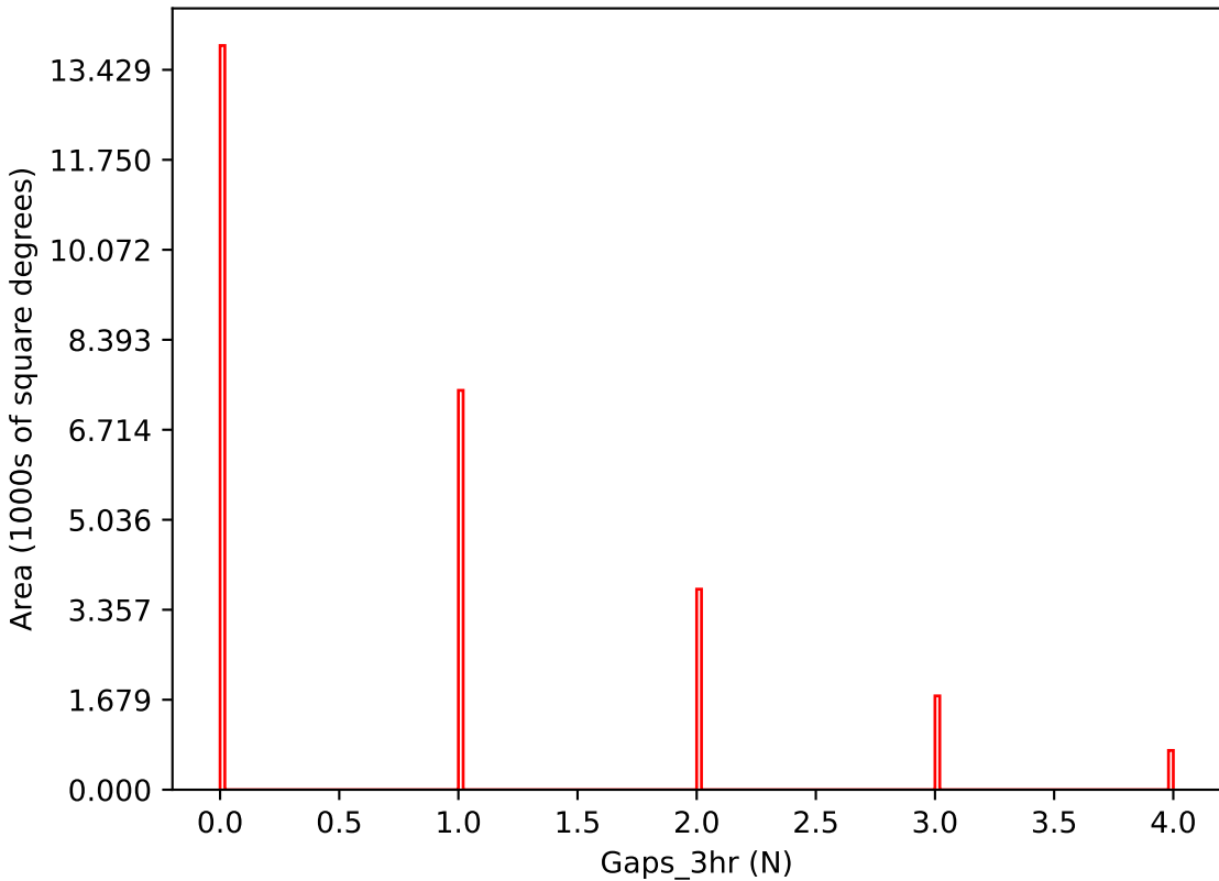
too_ignore_100_1v3.4_10yrs i band: Gaps_3hr
