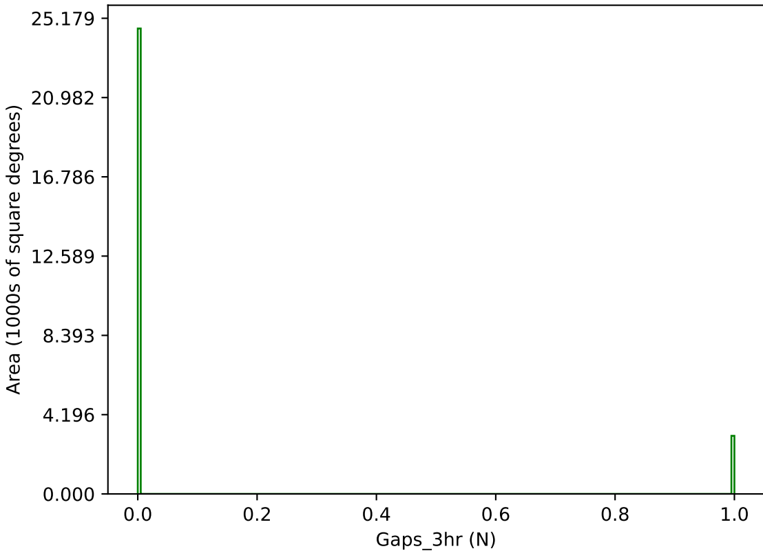
too_ignore_100_1v3.4_10yrs g band: Gaps_3hr
