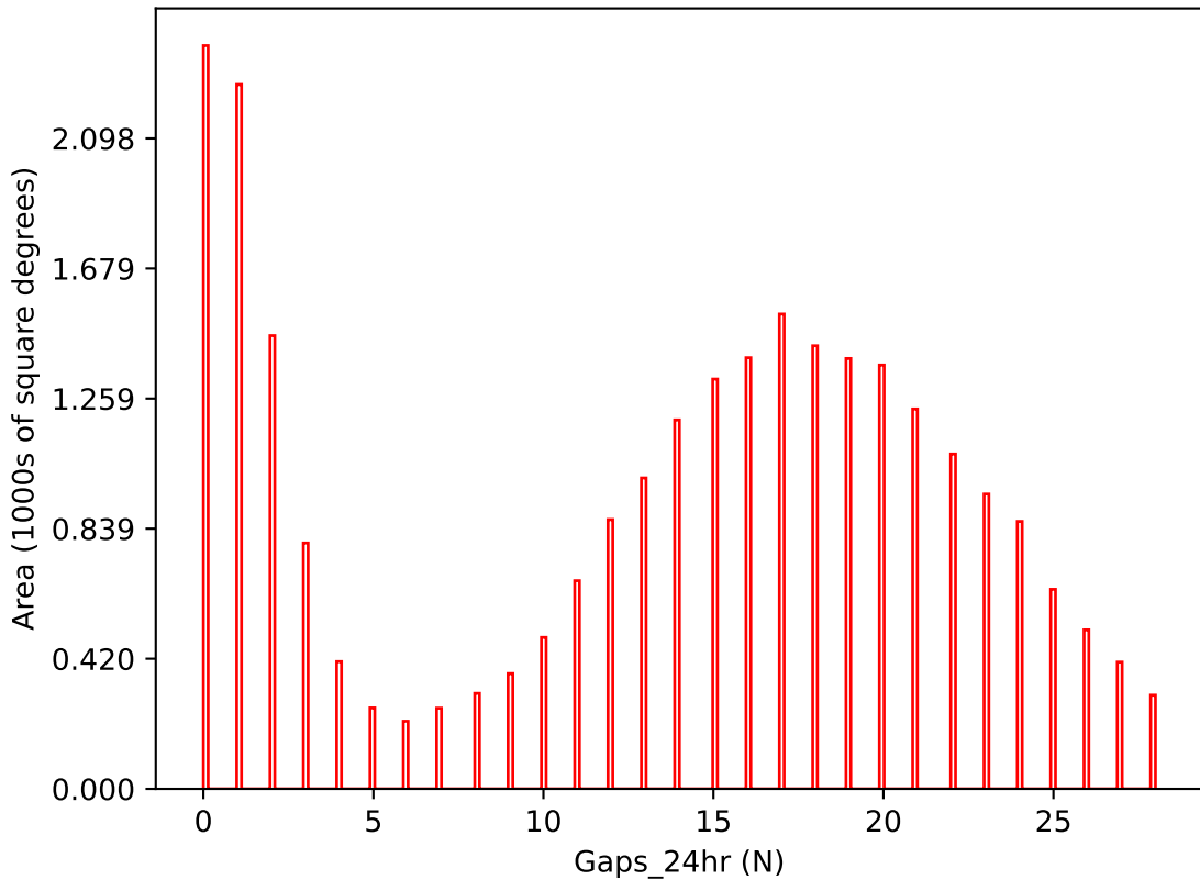
too_ignore_100_1v3.4_10yrs i band: Gaps_24hr
