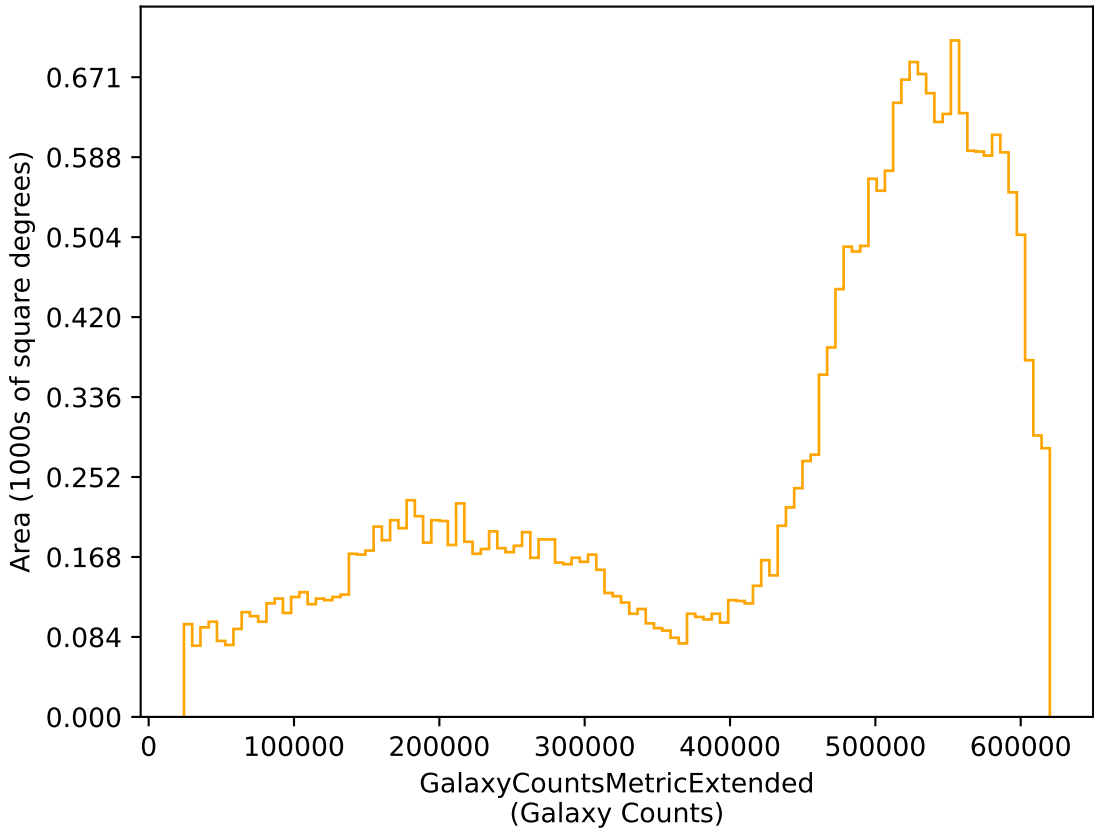
too_ignore_100_1v3.4_10yrs r: GalaxyCountsMetricExtended
