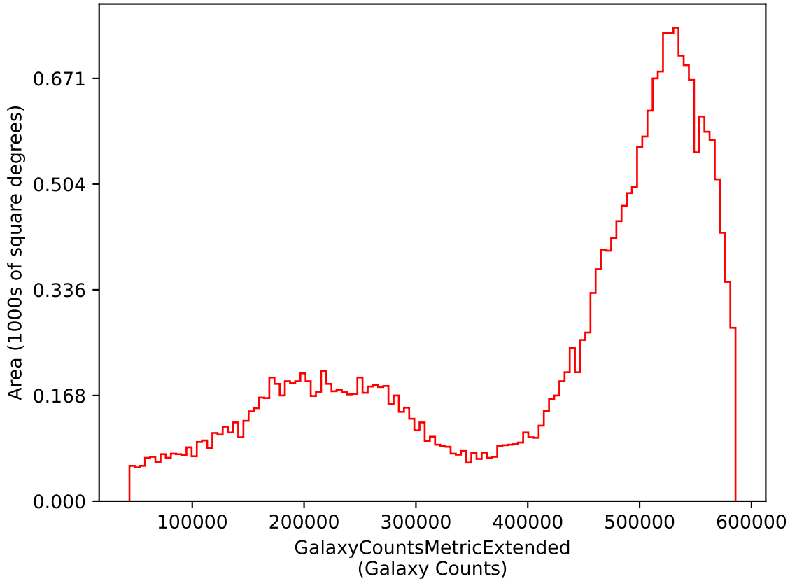
too_ignore_100_1v3.4_10yrs i: GalaxyCountsMetricExtended
