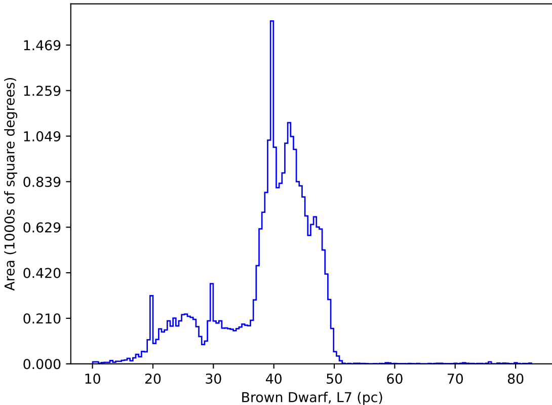
too_ignore_100_1v3.4_10yrs : Brown Dwarf, L7
