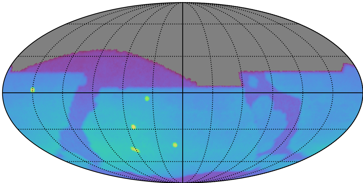
too_ignore_100_1v3.4_10yrs : Brown Dwarf, L4
