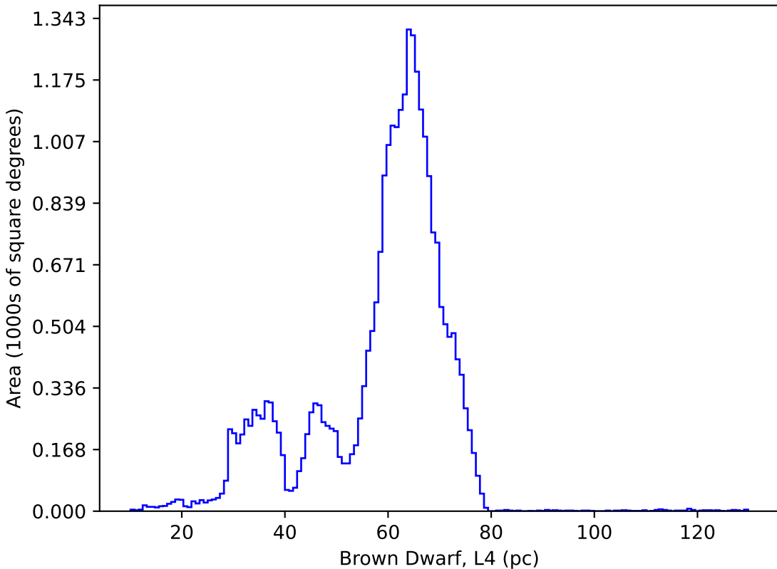
too_ignore_100_1v3.4_10yrs : Brown Dwarf, L4
