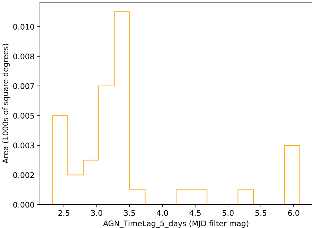
too_ignore_100_1v3.4_10yrs r band: AGN_TimeLag_5_days
