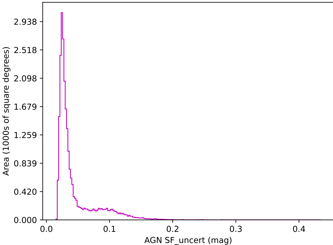
too_ignore_100_1v3.4_10yrs z band: AGN SF_uncert
