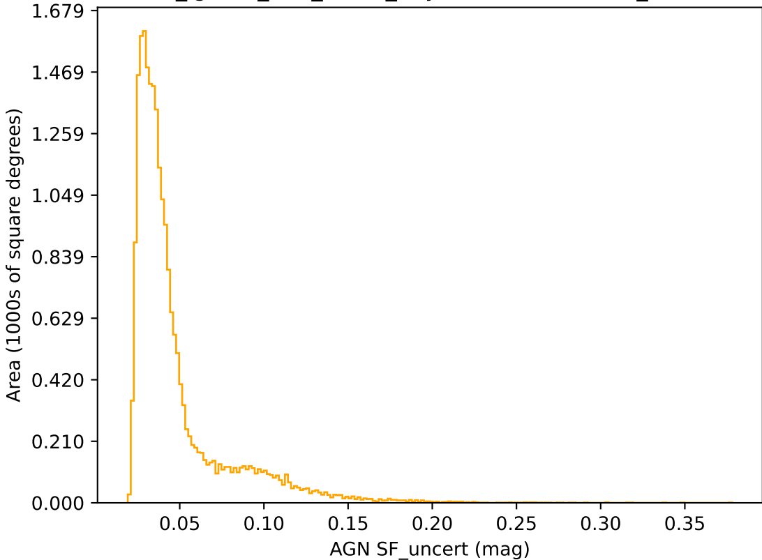
too_ignore_100_1v3.4_10yrs r band: AGN SF_uncert
