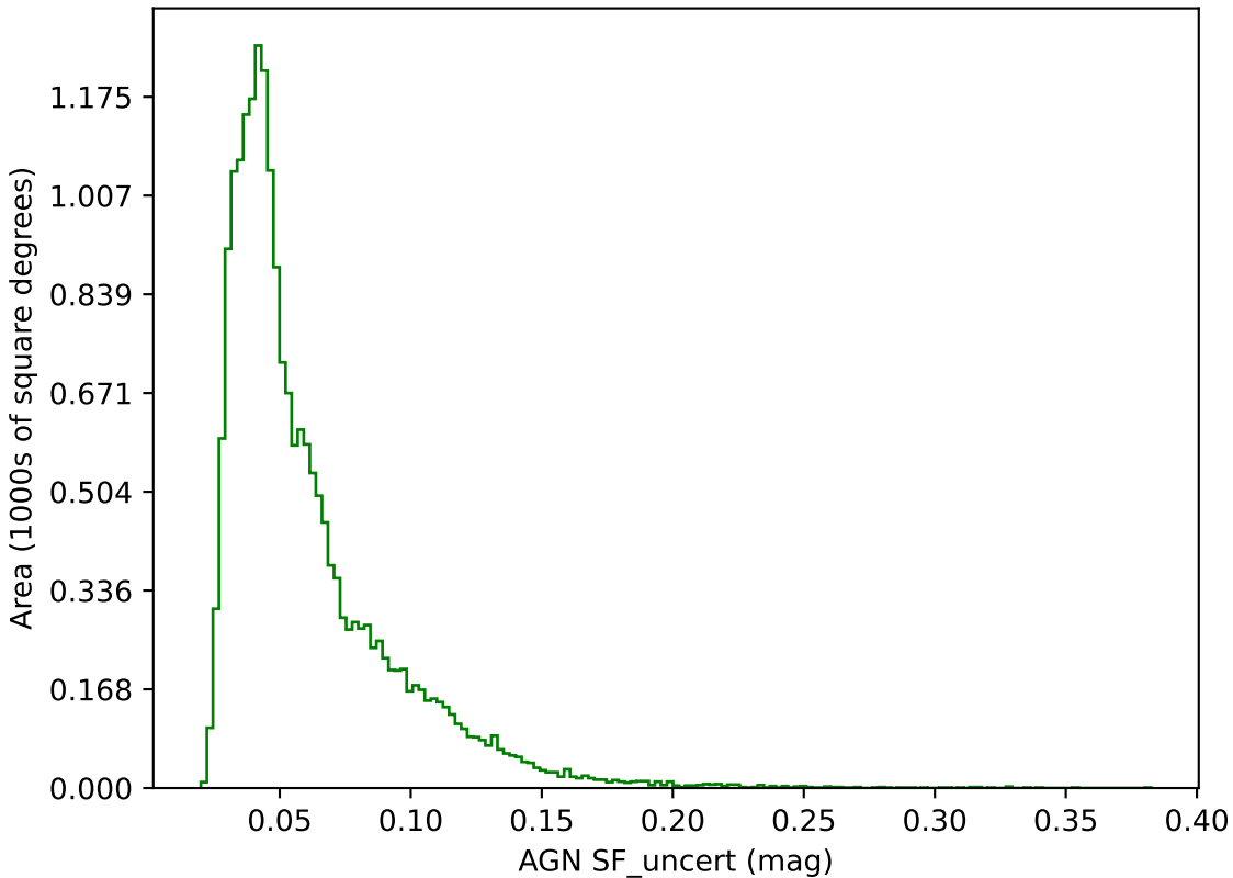
too_ignore_100_1v3.4_10yrs g band: AGN SF_uncert
