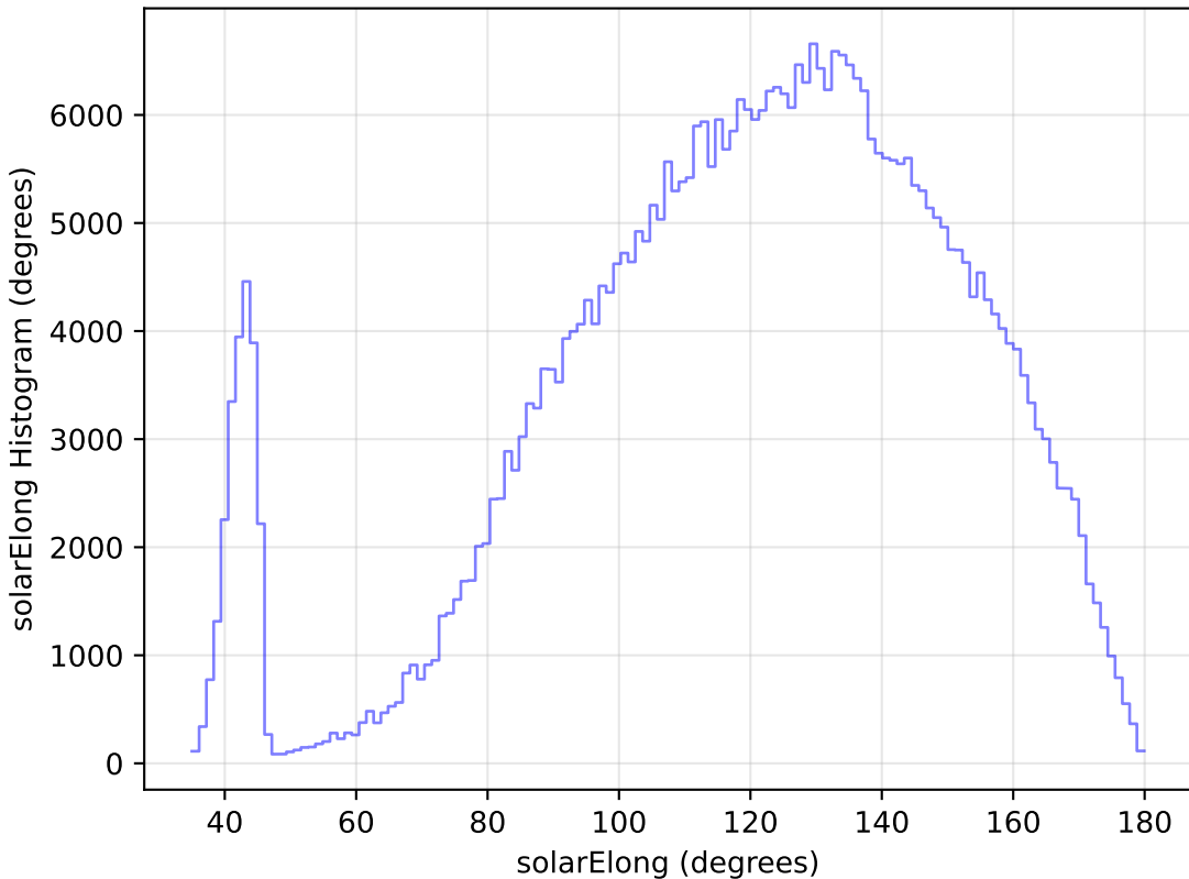
too_ignore_100_1v3.4_10yrs WFD z band: solarElong Histogram
