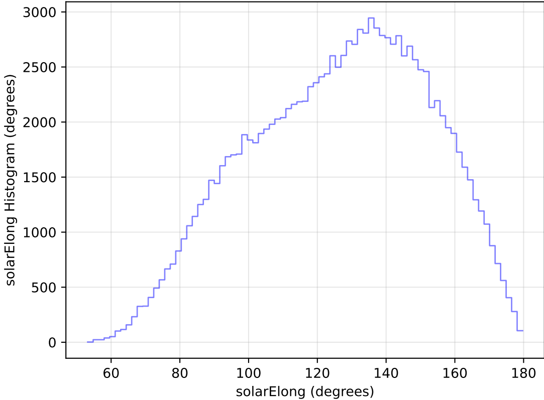
too_ignore_100_1v3.4_10yrs WFD u band: solarElong Histogram
