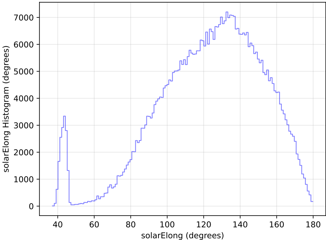
too_ignore_100_1v3.4_10yrs WFD r band: solarElong Histogram
