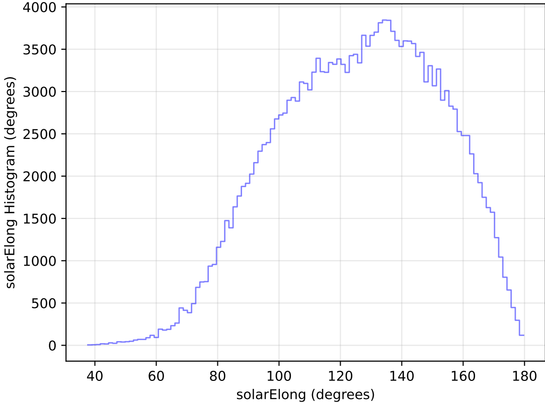
too_ignore_100_1v3.4_10yrs WFD g band: solarElong Histogram
