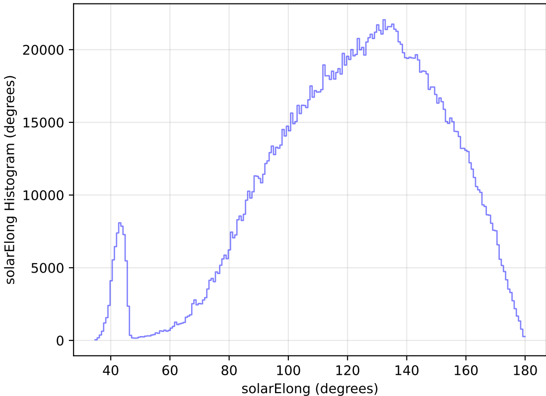
too_ignore_100_1v3.4_10yrs WFD all bands: solarElong Histogram
