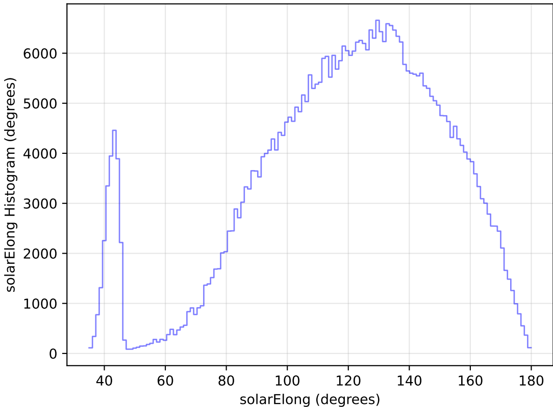
too_ignore_100_1v3.4_10yrs All sky z band: solarElong Histogram
