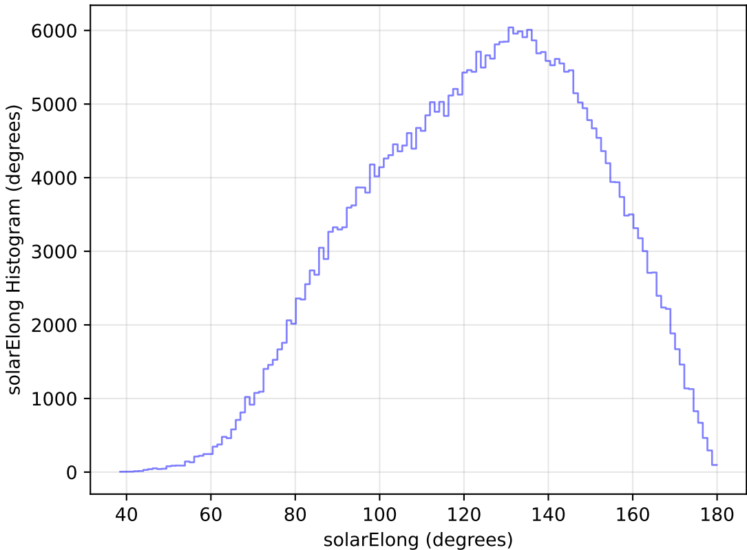
too_ignore_100_1v3.4_10yrs All sky y band: solarElong Histogram
