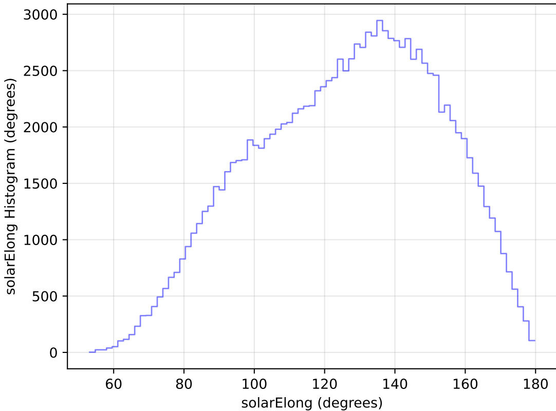
too_ignore_100_1v3.4_10yrs All sky u band: solarElong Histogram
