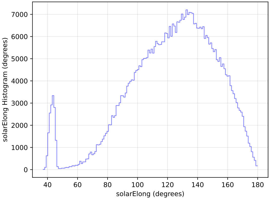
too_ignore_100_1v3.4_10yrs All sky r band: solarElong Histogram
