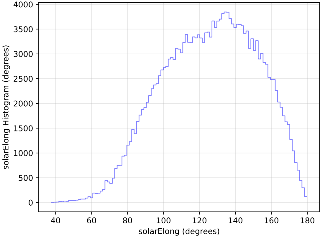
too_ignore_100_1v3.4_10yrs All sky g band: solarElong Histogram
