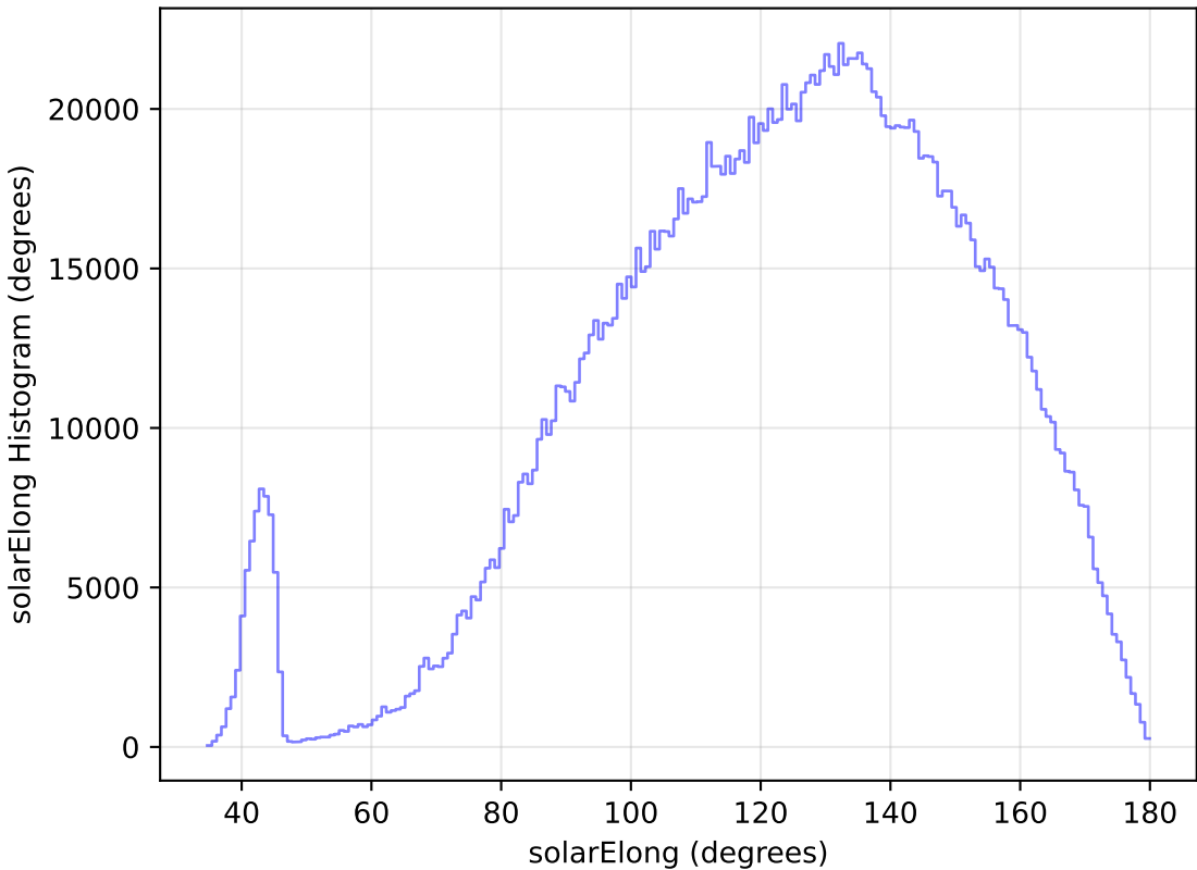
too_ignore_100_1v3.4_10yrs All sky all bands: solarElong Histogram
