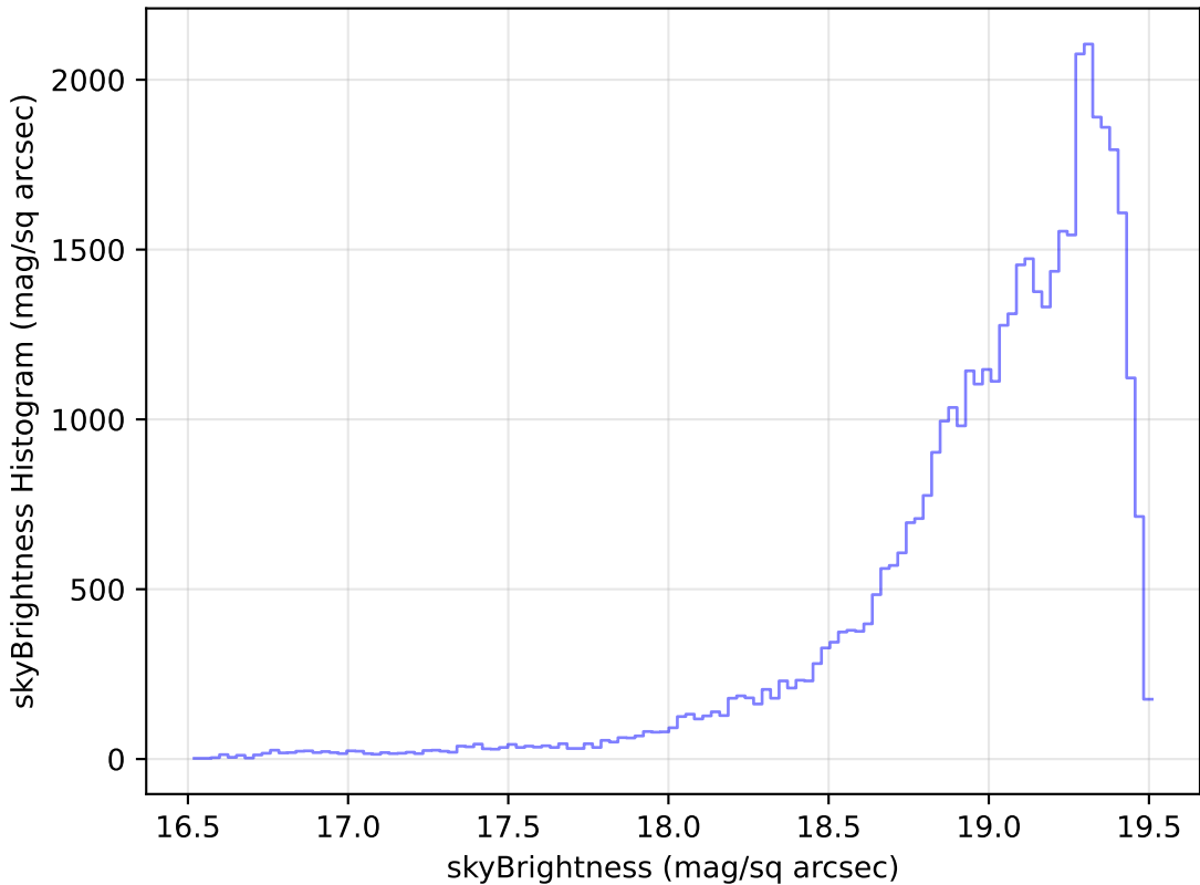
too_ignore_100_1v3.4_10yrs Yr 1 z band: skyBrightness Histogram
