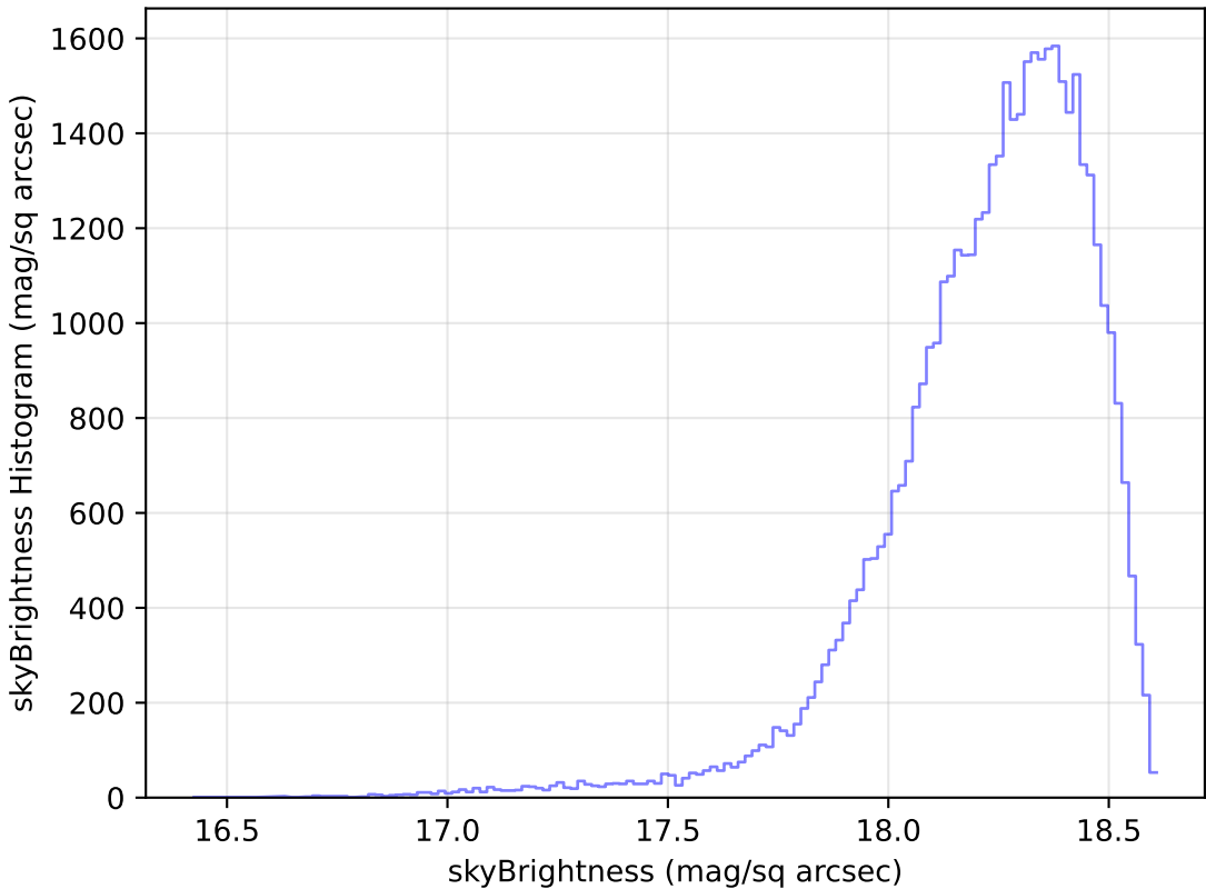
too_ignore_100_1v3.4_10yrs Yr 1 y band: skyBrightness Histogram
