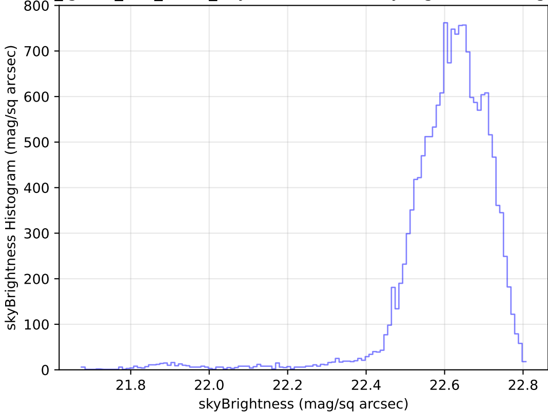
too_ignore_100_1v3.4_10yrs Yr 1 u band: skyBrightness Histogram
