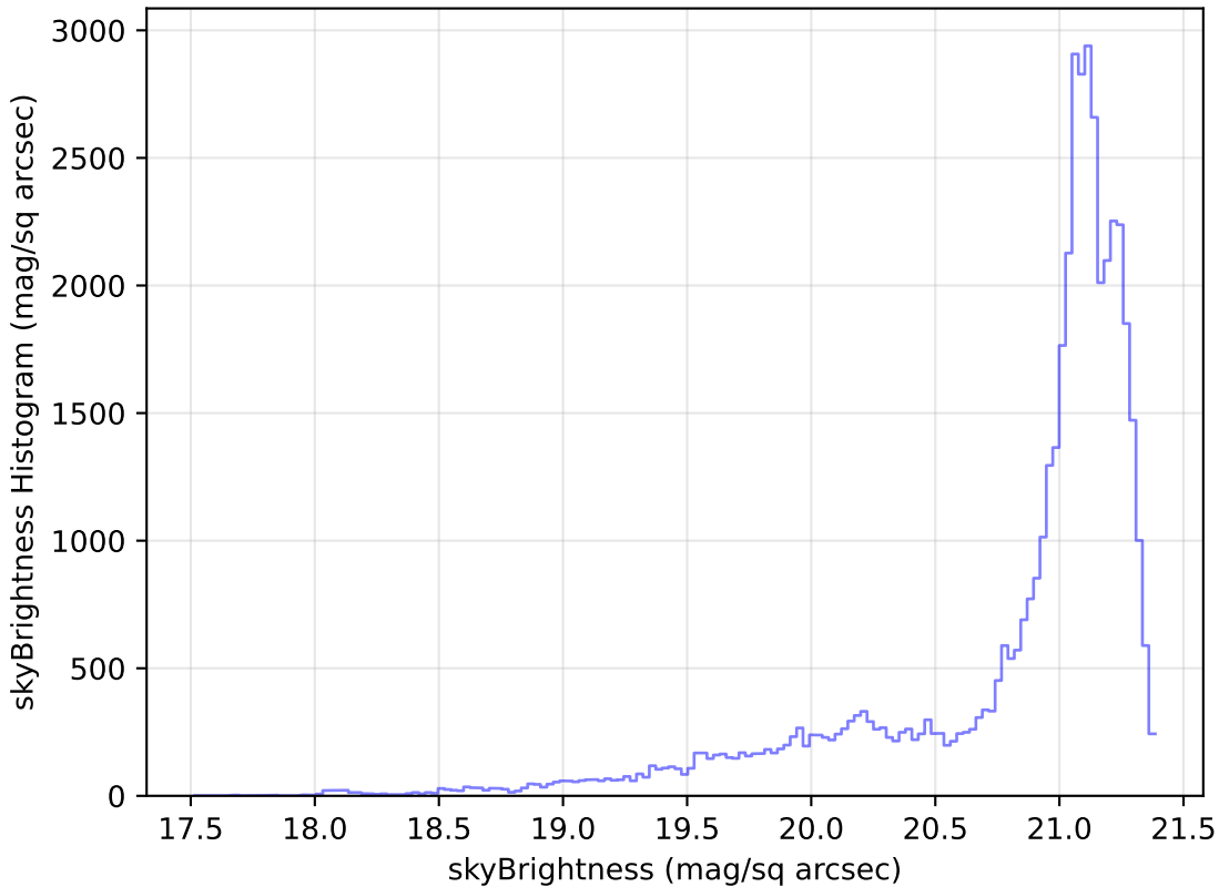
too_ignore_100_1v3.4_10yrs Yr 1 r band: skyBrightness Histogram
