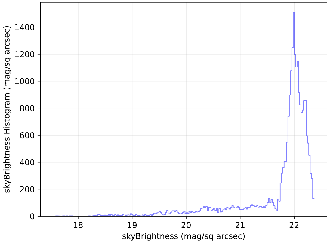
too_ignore_100_1v3.4_10yrs Yr 1 g band: skyBrightness Histogram
