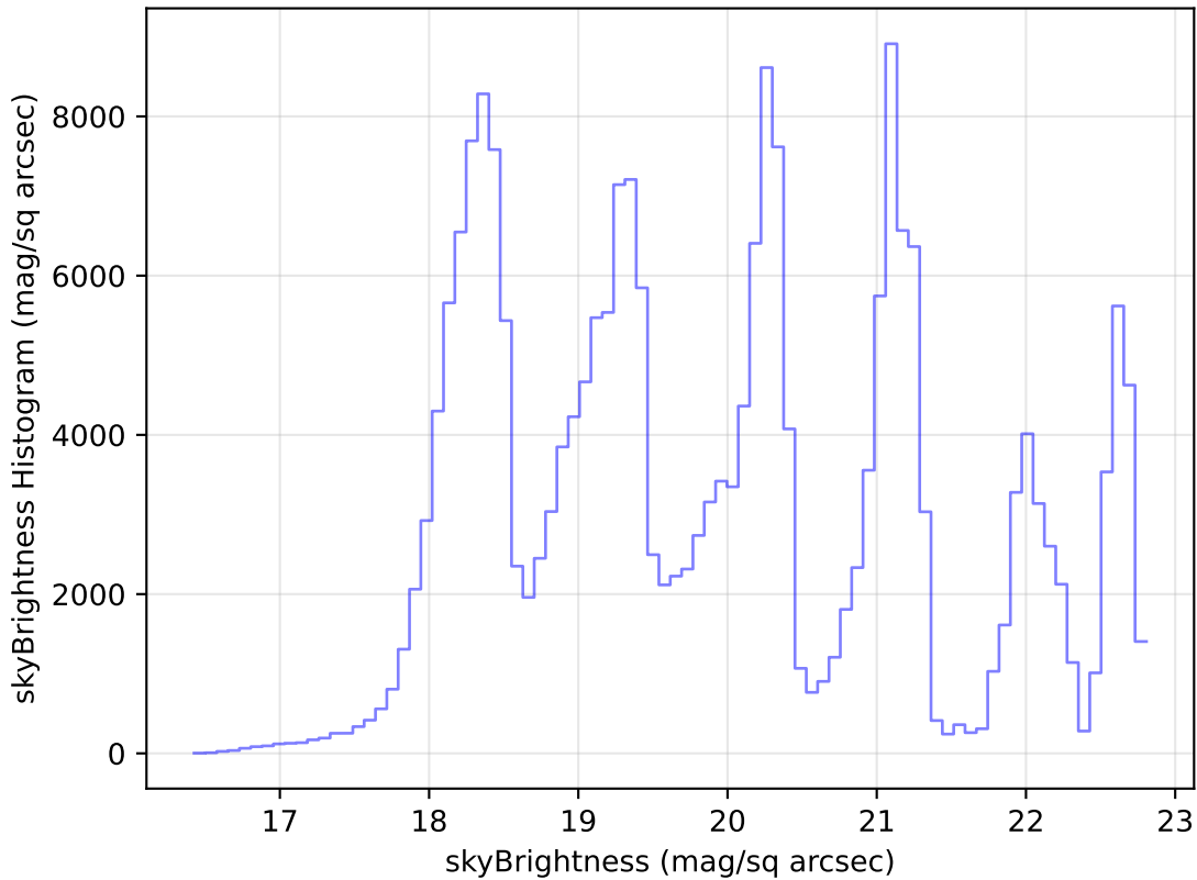
too_ignore_100_1v3.4_10yrs Yr 1 all bands: skyBrightness Histogram
