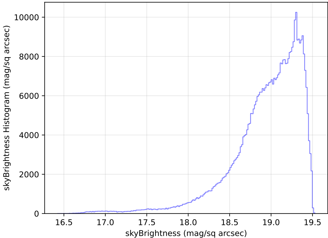
too_ignore_100_1v3.4_10yrs WFD z band: skyBrightness Histogram
