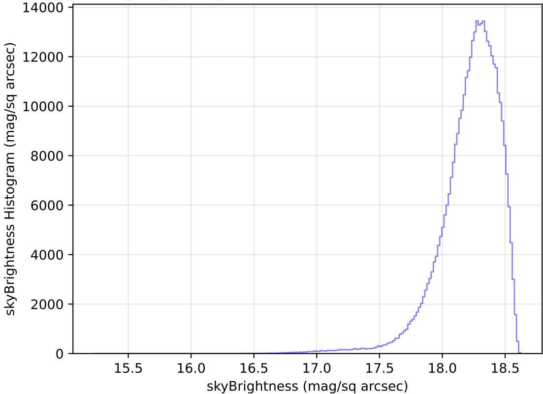
too_ignore_100_1v3.4_10yrs WFD y band: skyBrightness Histogram
