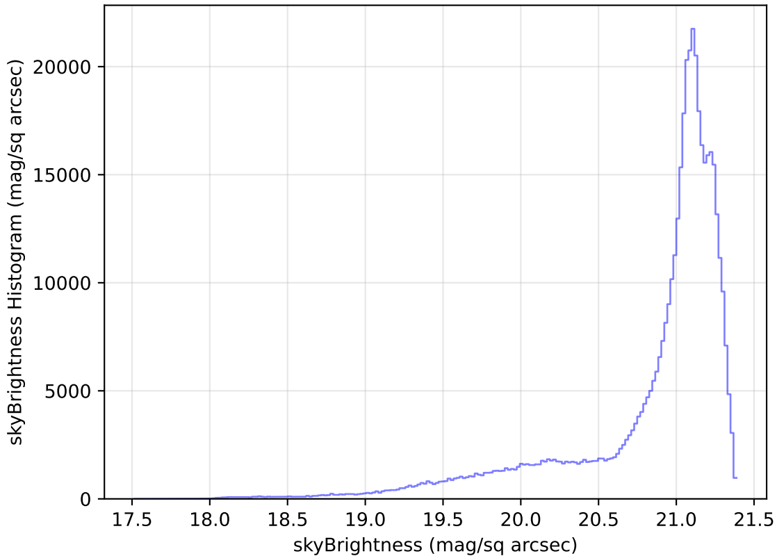
too_ignore_100_1v3.4_10yrs WFD r band: skyBrightness Histogram
