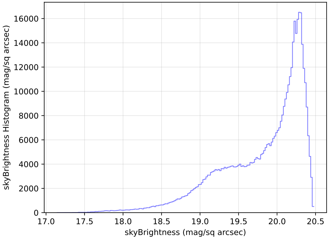
too_ignore_100_1v3.4_10yrs WFD i band: skyBrightness Histogram
