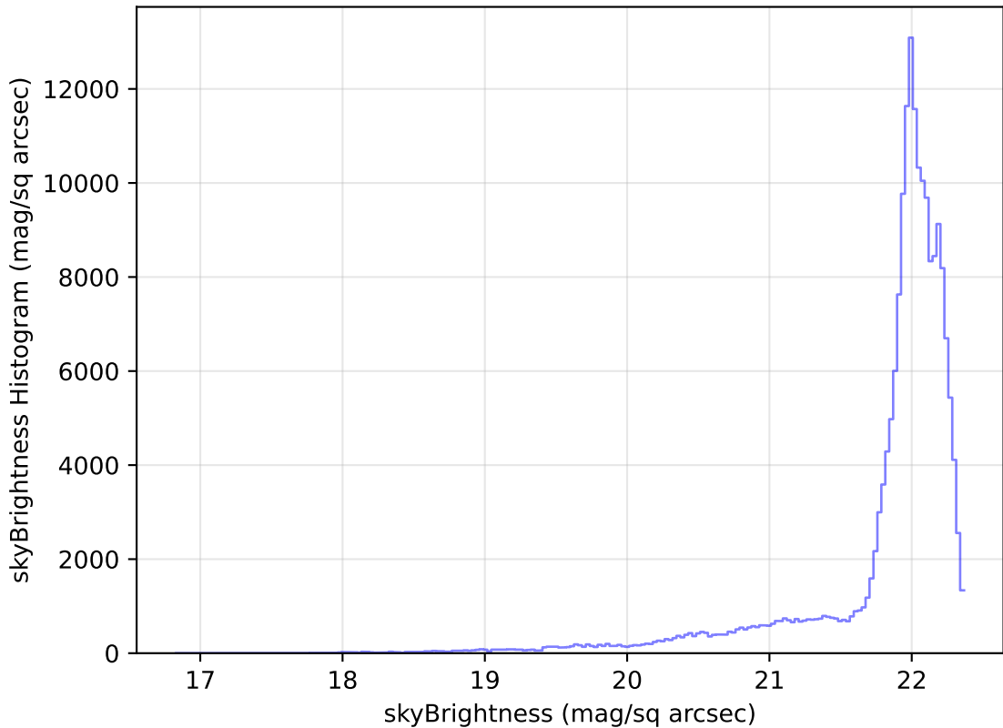
too_ignore_100_1v3.4_10yrs WFD g band: skyBrightness Histogram
