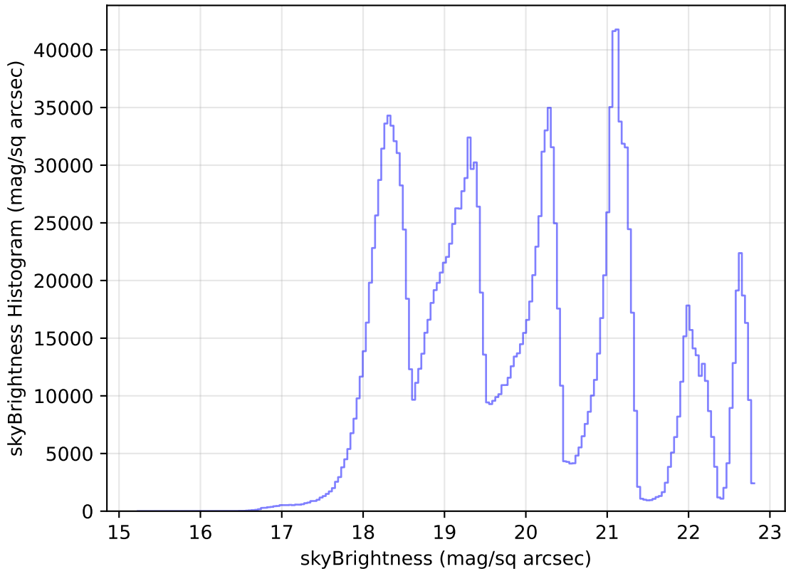
too_ignore_100_1v3.4_10yrs WFD all bands: skyBrightness Histogram
