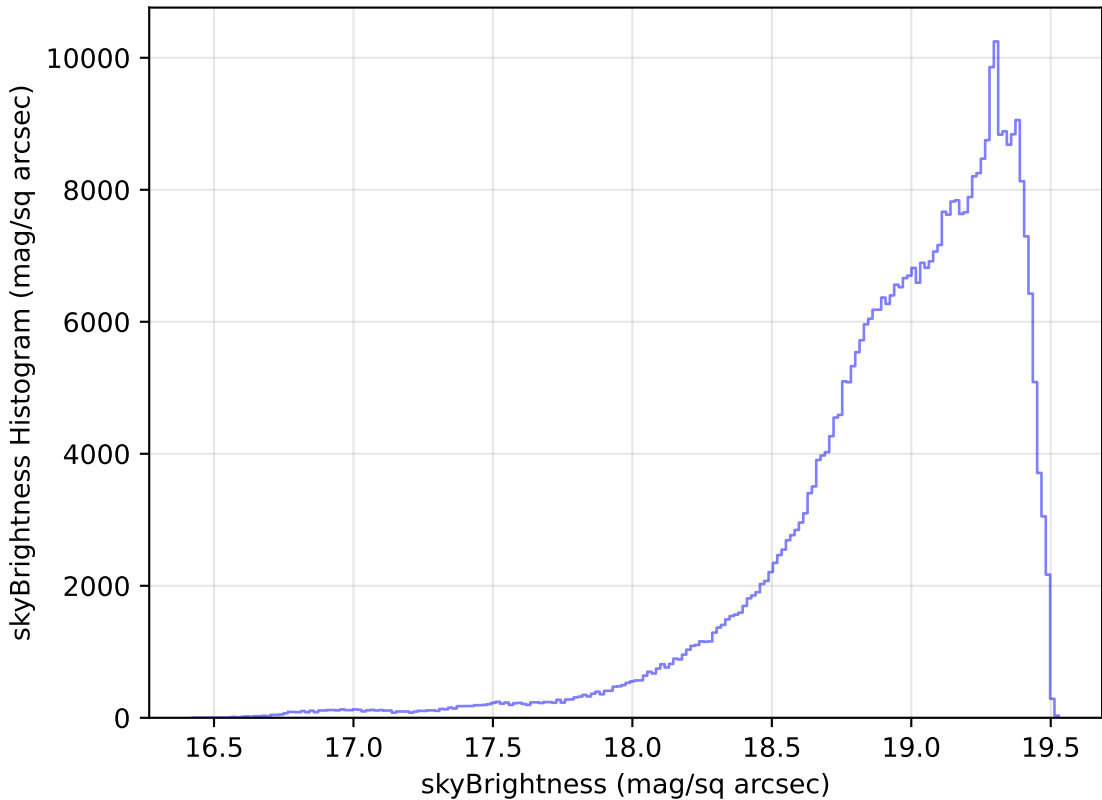
too_ignore_100_1v3.4_10yrs All sky z band: skyBrightness Histogram
