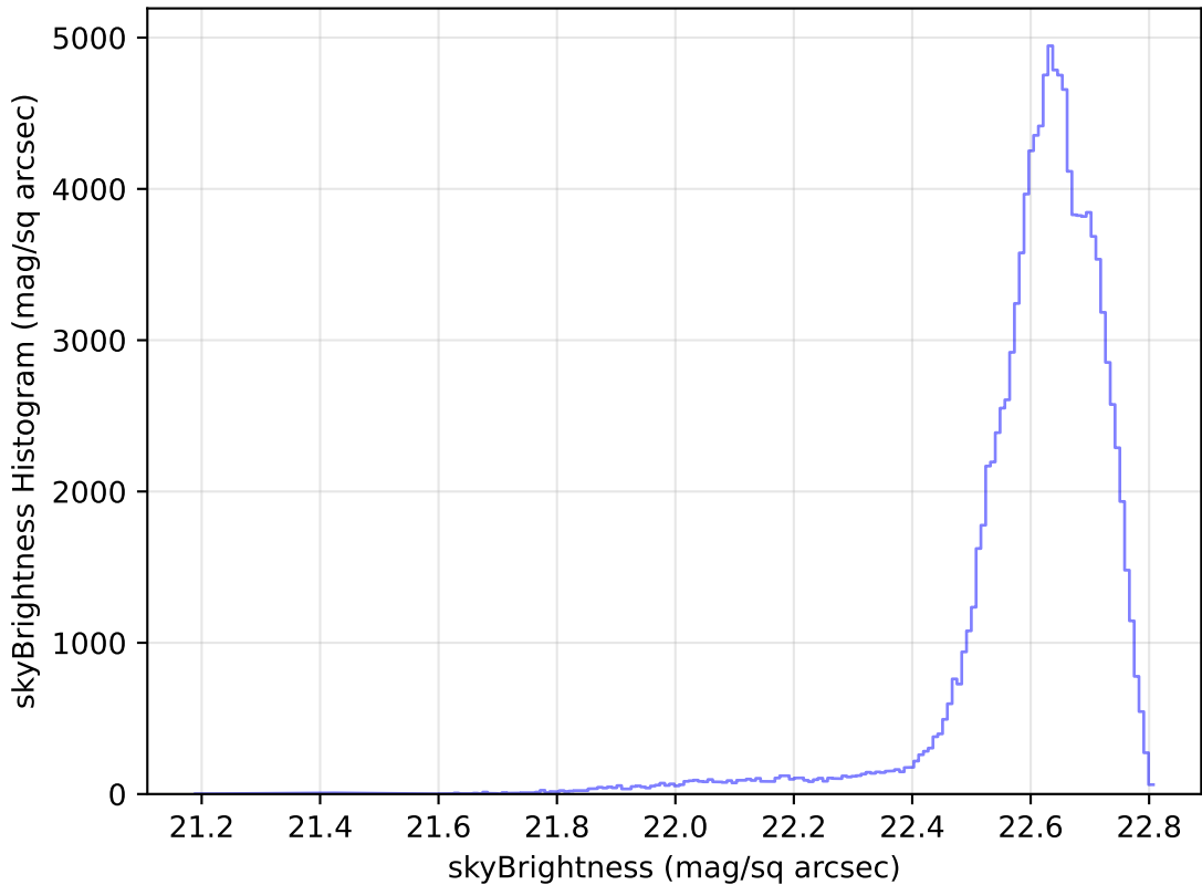
too_ignore_100_1v3.4_10yrs All sky u band: skyBrightness Histogram
