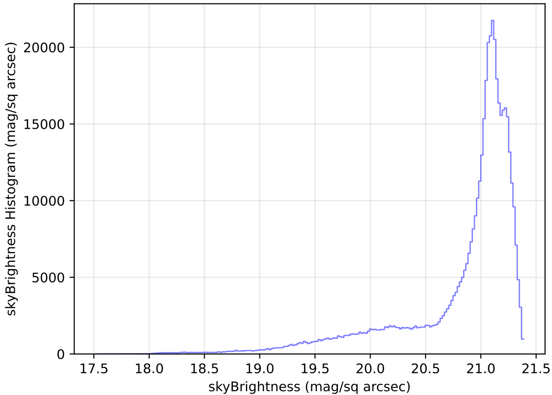
too_ignore_100_1v3.4_10yrs All sky r band: skyBrightness Histogram
