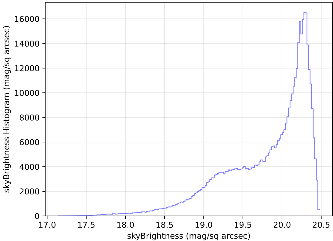
too_ignore_100_1v3.4_10yrs All sky i band: skyBrightness Histogram
