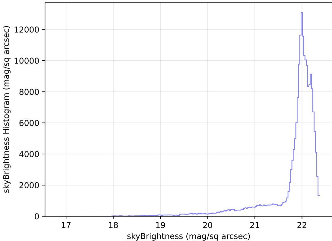
too_ignore_100_1v3.4_10yrs All sky g band: skyBrightness Histogram
